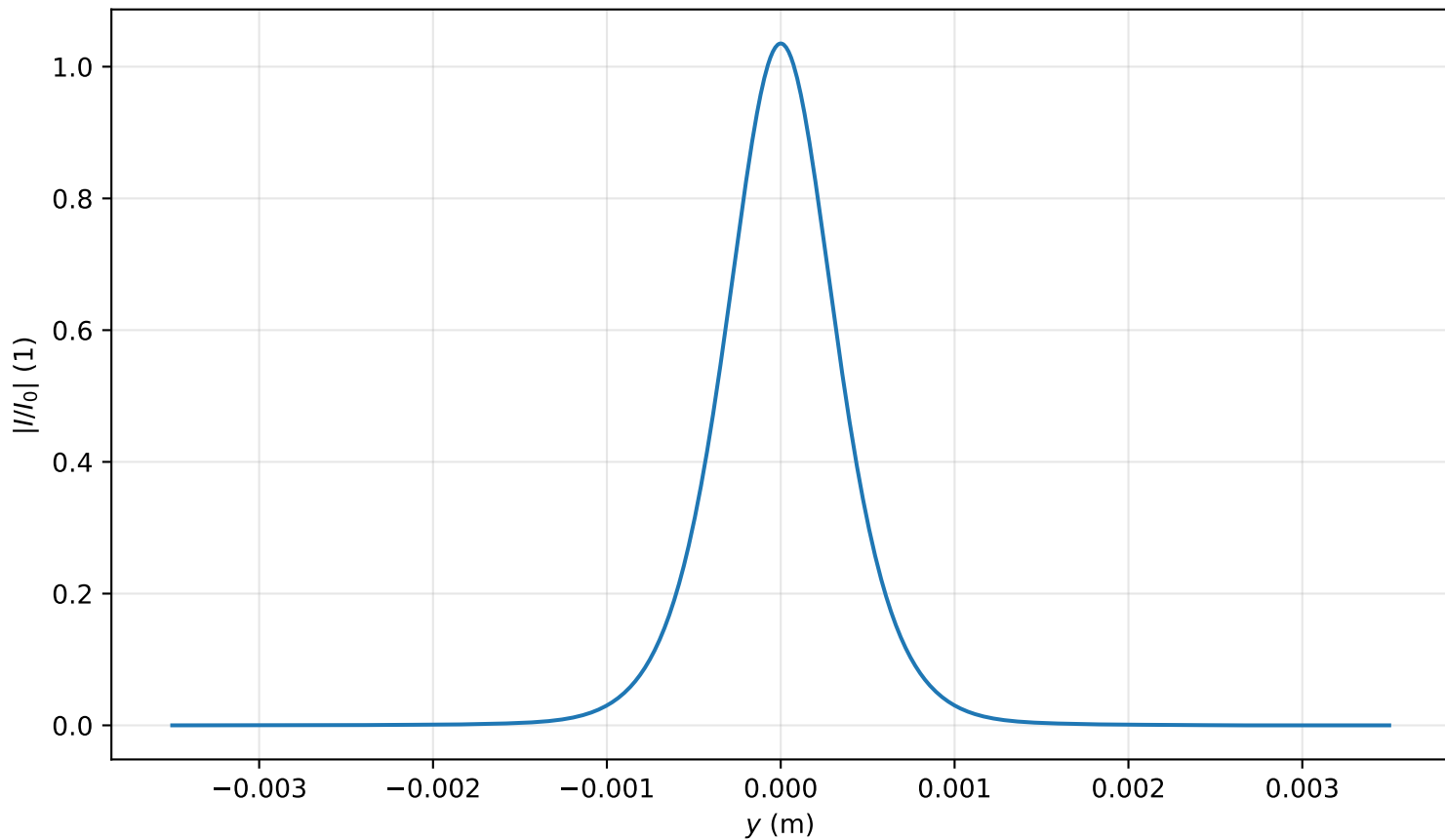
Intensity profile I(x=0, y, z=3.264)/I_0 , P_{in}=0.8P_{cr} , artificial time
